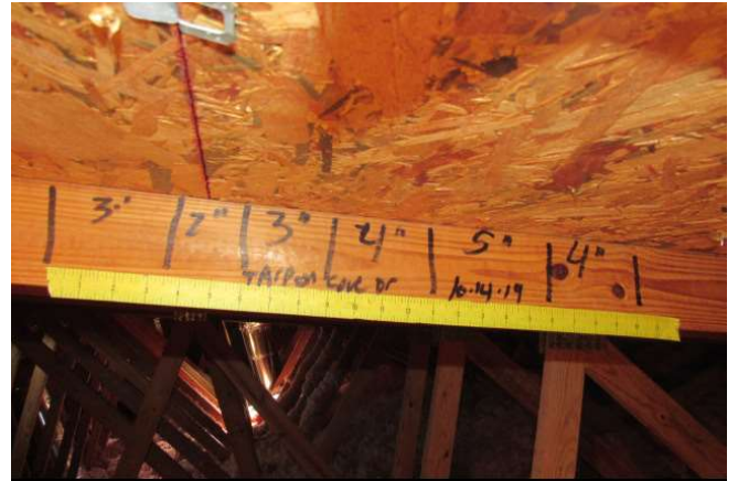
Roof Deck Connection - Nail Spacing #1
