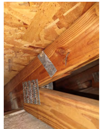
Roof to Wall Connection Single Wrap Back
