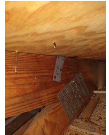
Roof to Wall Connection Single Wrap Back
