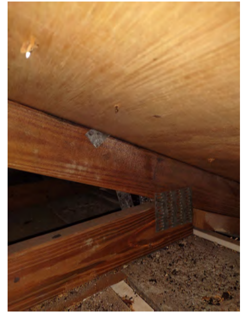
Roof to Wall Connection Single Wrap Back
